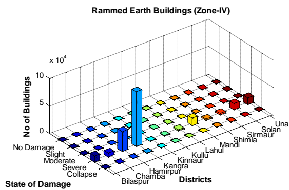
Figure 106: Damage state of rammed earth buildings in all districts of HP subjected to 0.24 g & 0.36g
