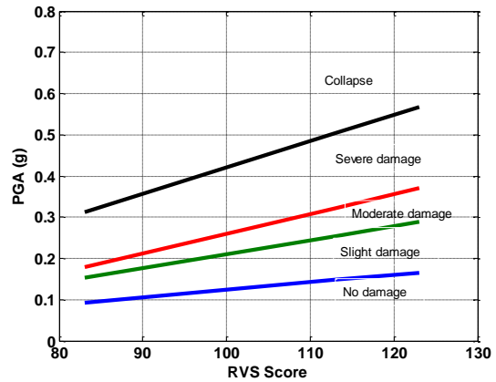
(b) Brick masonry buildings
