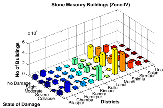
Figure 105: Damage state of stone masonry buildings in all districts of HP subjected to 0.24 g & 0.36g
