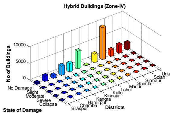
Figure 107: Damage state of hybrid buildings in all districts of HP subjected to 0.24 g & 0.36g
