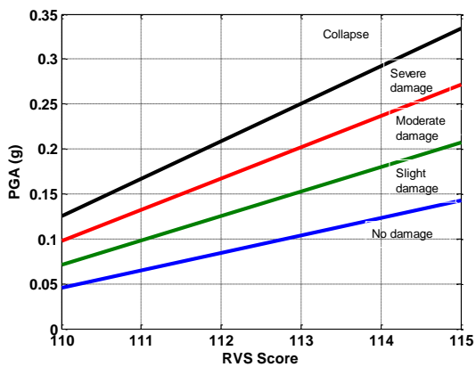
(c) Stone masonry buildings
