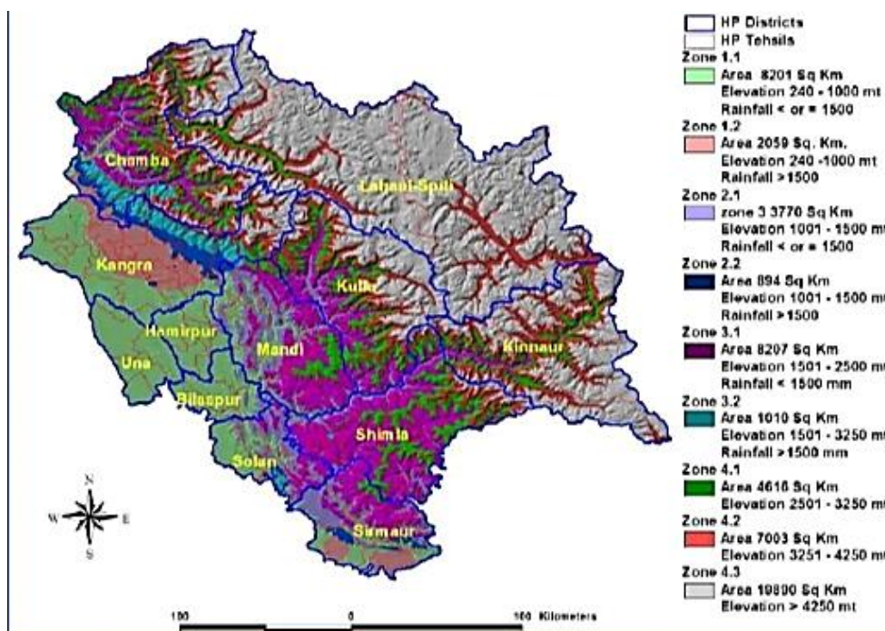
Figure 4: Redefined Agro-Ecological Zone
