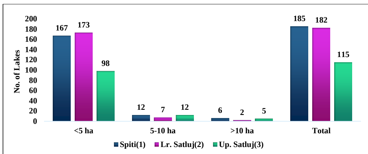
Fig. 7.2 (b): No of lakes based on IRS-R2, LISS III, 96/48 and 96/49
