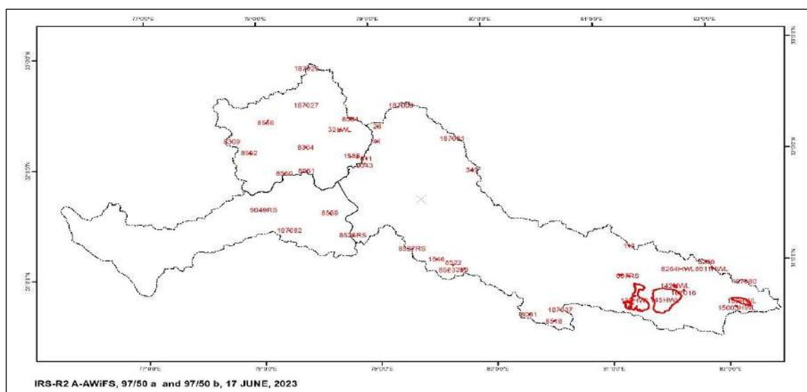
Fig. 6.3 (b): IRS-R2-AWiFS, 97/50 A and 97/50 B, 17 th June, 2023, Interpreted Layers
