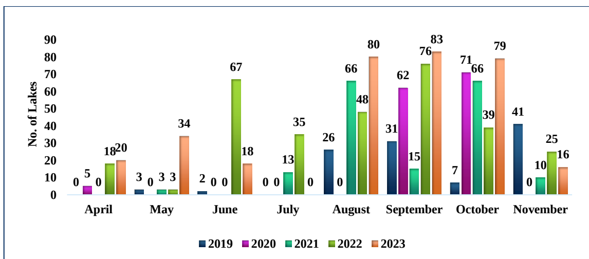
Fig. 8.4: Total No. of Lakes > 10ha based on AWiFS satellite data (2019- 2023)
