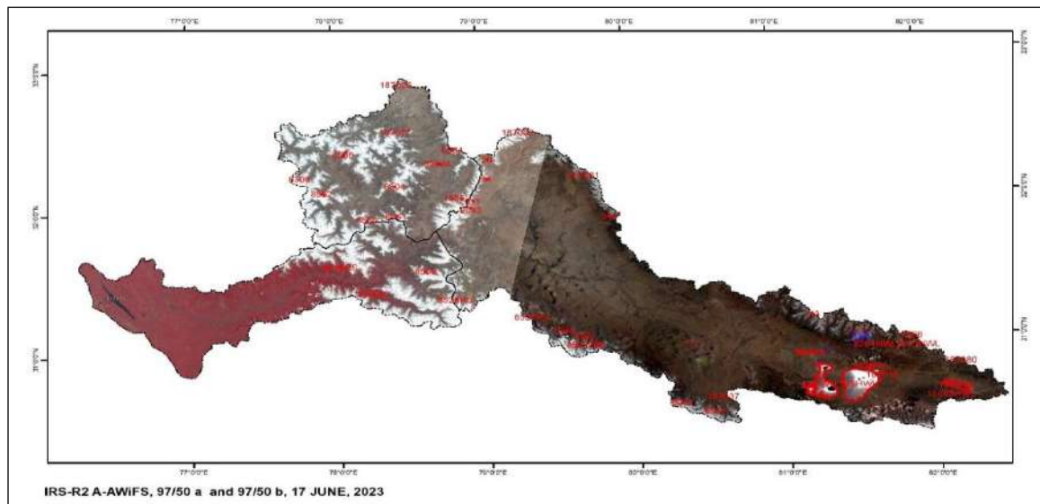
Fig. 6.3 (a): IRS-R2-AWiFS, 97/50 A and 97/50 B, 17 th June 2023
