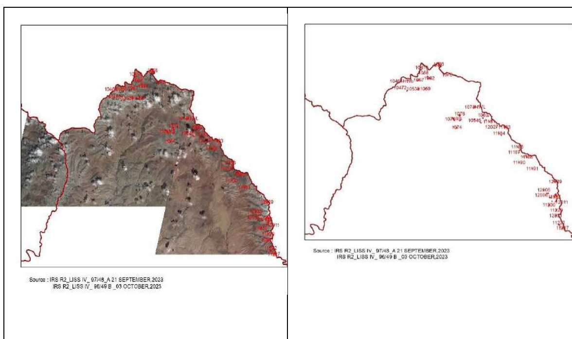
Fig. 9.4 (a) & (b): IRS R2, LISS IV, 97/48 a, 21 September and 97/4b, 03 October and its interpreted layer
