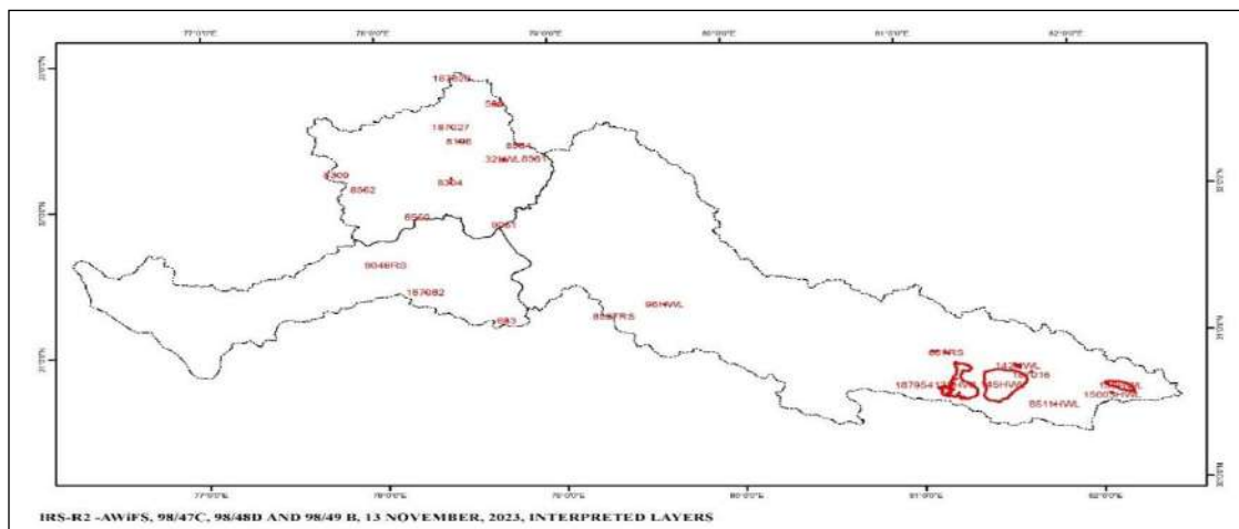
Fig. 6.8 (f): IR, R2-AWiFS, 13 th November, 2023, Interpreted Layers
