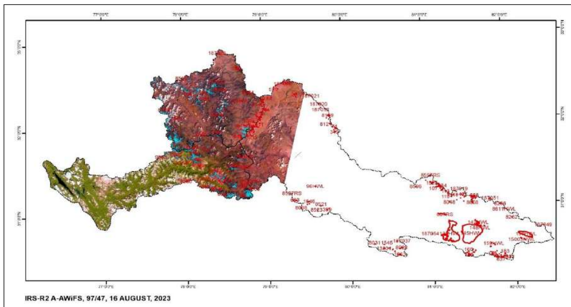
Fig. 6.5 (a): IRS-R2 -AWiFS, 97/47, 16 AUGUST, 2023
