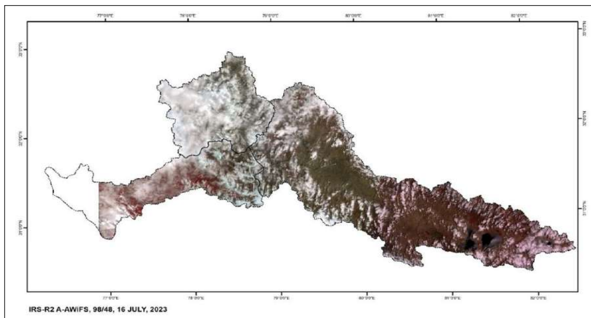
Fig. 7.4 (a): IRS-R2 A-AWiFS, 98/48, 16 th July, 2023
