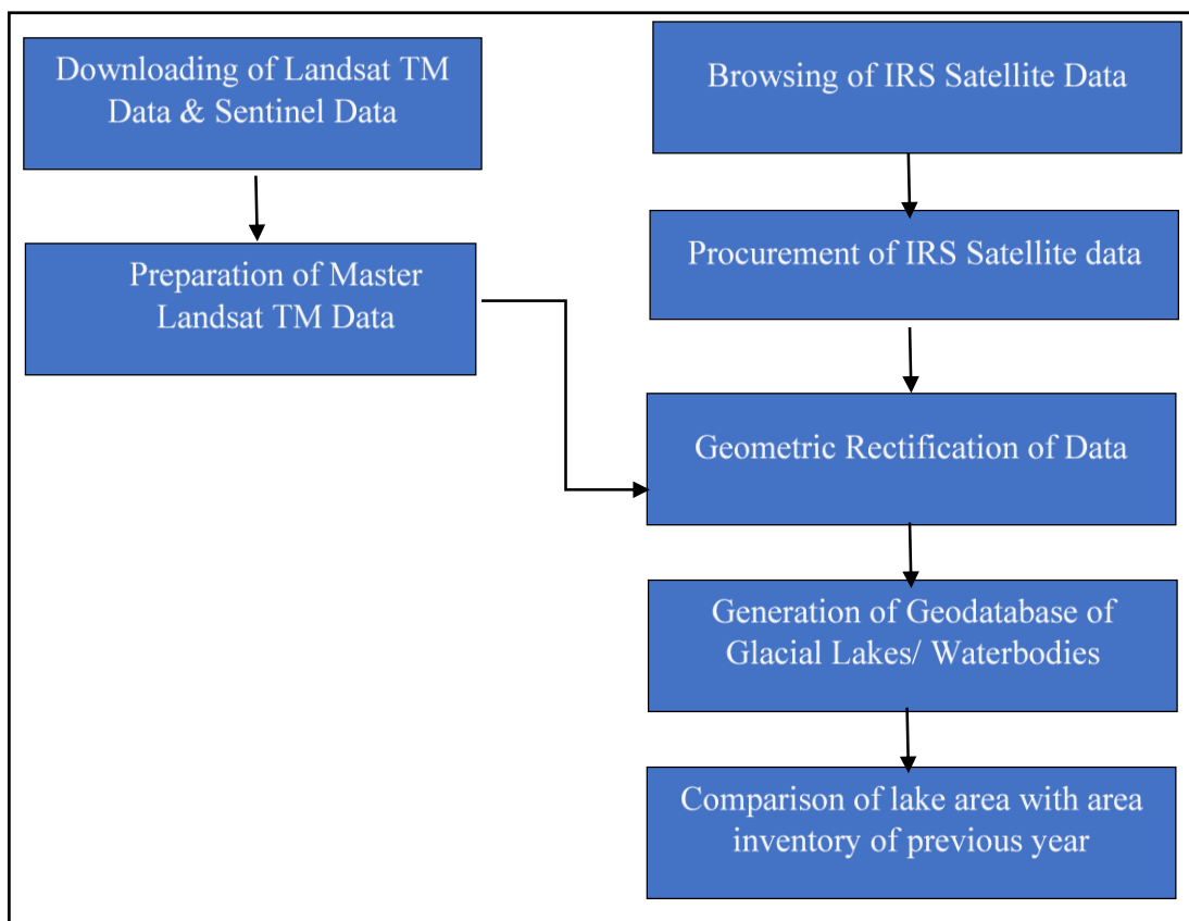
Fig. 4.1: Flow Chart Methodology
