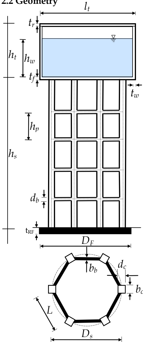
Figure 2.1: Elevated Water Tanks- Frame Staging
